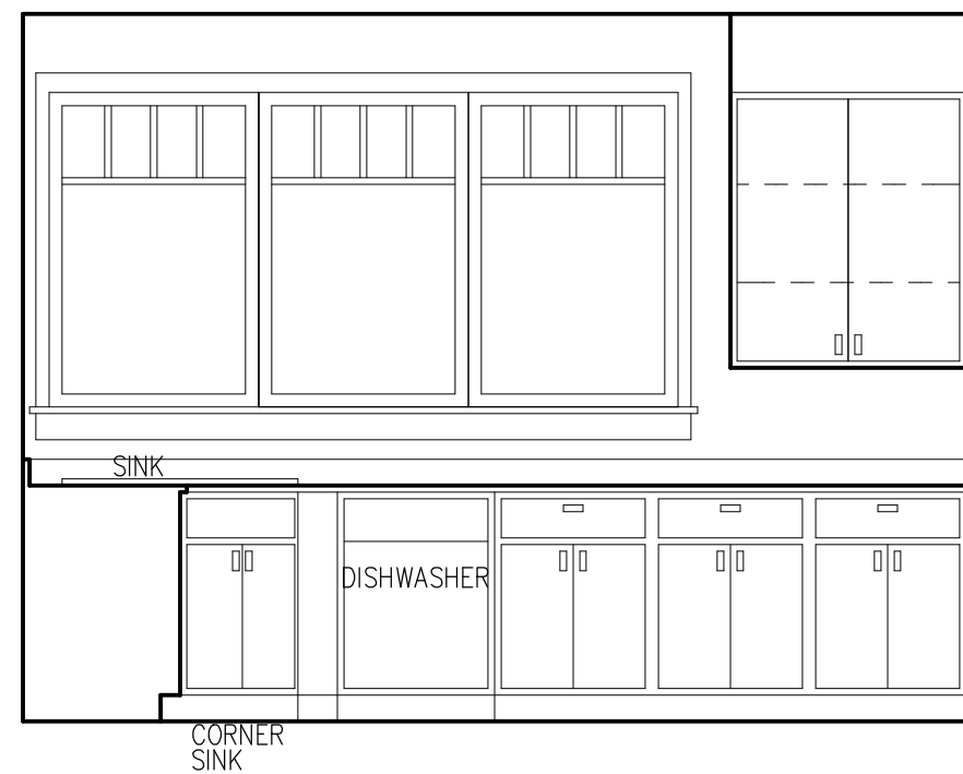
DISHWASHER ELEVATION
