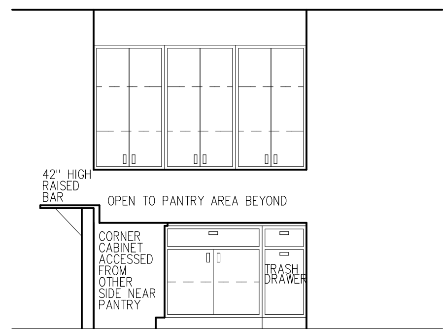
RAISED BAR ELEVATION
